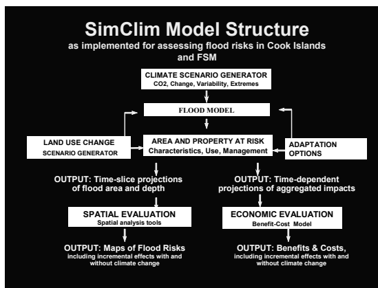
Figure 7. SimCLIM structure as developed for coastal flood risk analyses and applied in the Cook Islands case study
